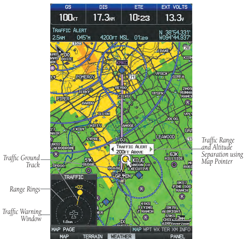
TIS (Map Page)
