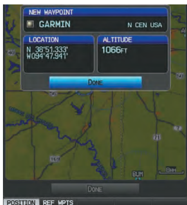
New Waypoint Window (POSITION Softkey Selected)
